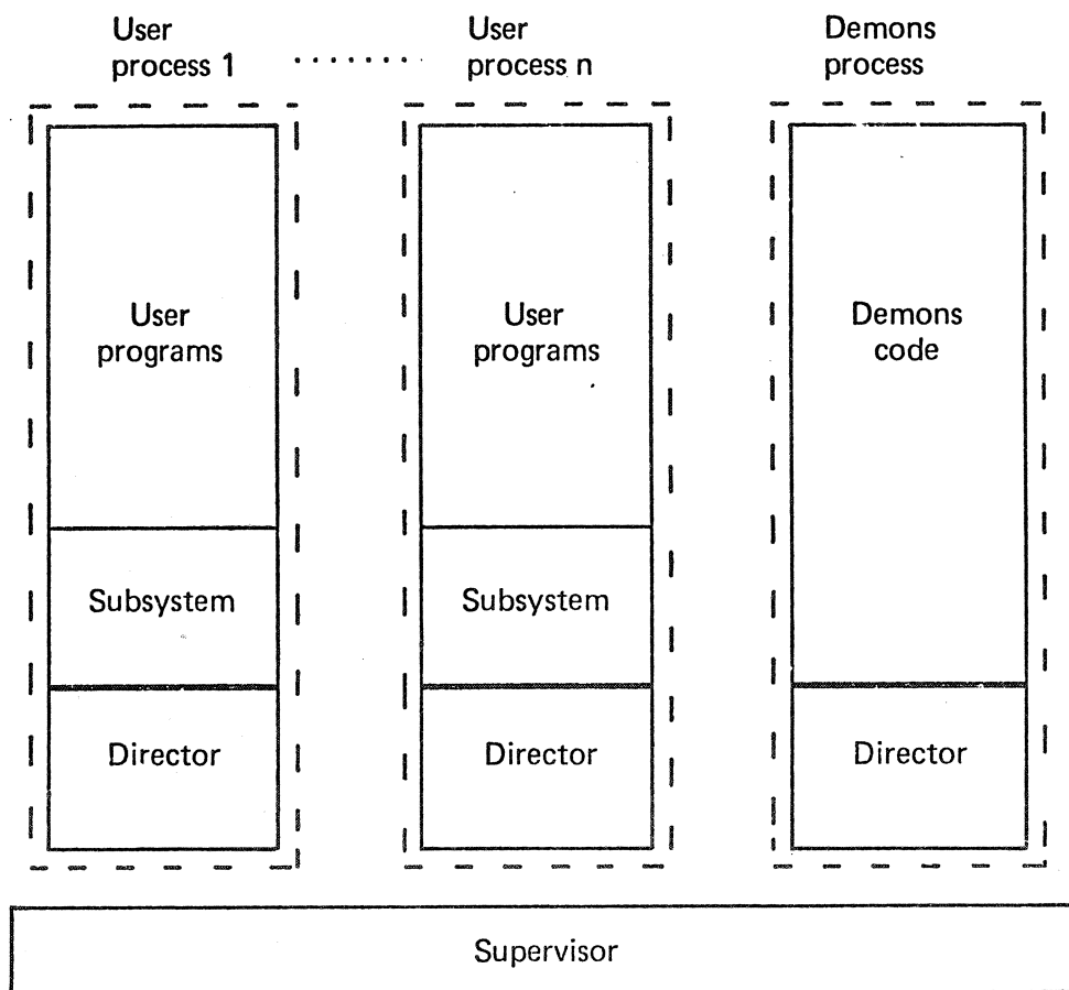
Fig. 1 Conceptual organisation of EMAS processes.
