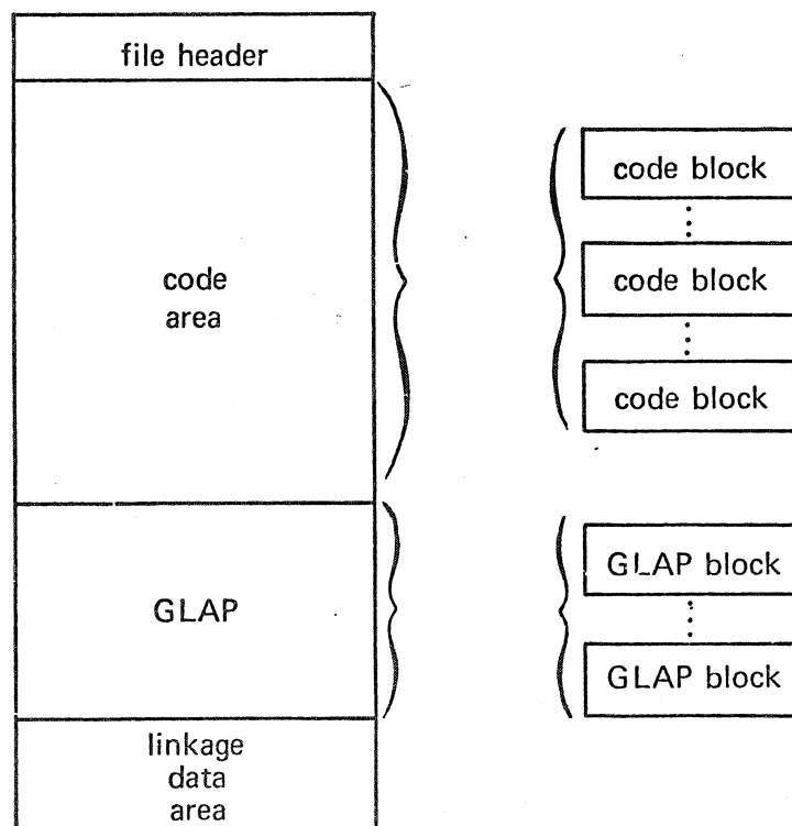
Fig. 3 Program file format
