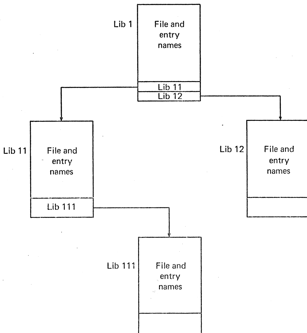
Fig. 5 Typical library index structure
